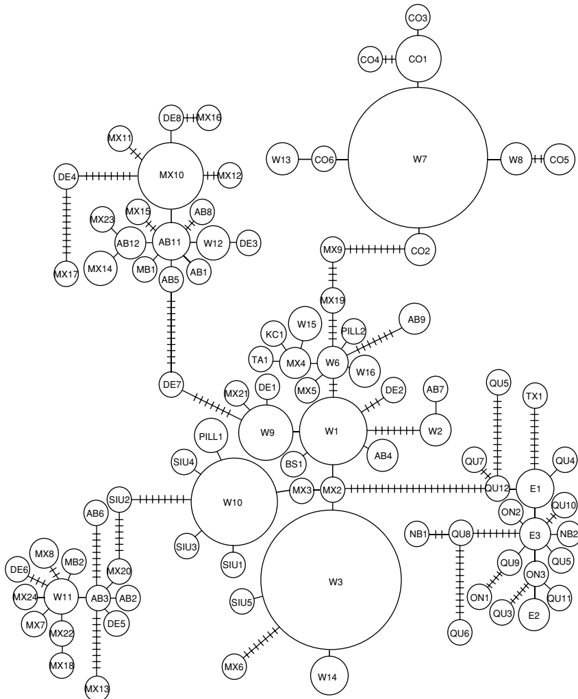
Fig. 2 Minimum spanning network for the 94 Wilson's warbler control region haplotypes. The size of the circle denoting each haplotype is proportional to the number of sequenced individuals with that haplotype. Hatch marks along branches indicate the inferred number of nucleotide substitutions separating haplotypes. Haplotype designations indicate location of origin (see Table 1 for site-specific abbreviations; W = haplotypes recovered from \geq 2 western breeding locations; E = haplotypes recovered from \geq 2 eastern breeding locations; MX = haplotypes recovered only from overwintering locations). The group of haplotypes at bottom right is the 'eastern group' referred to in the text; all other haplotypes fall in the western group.
