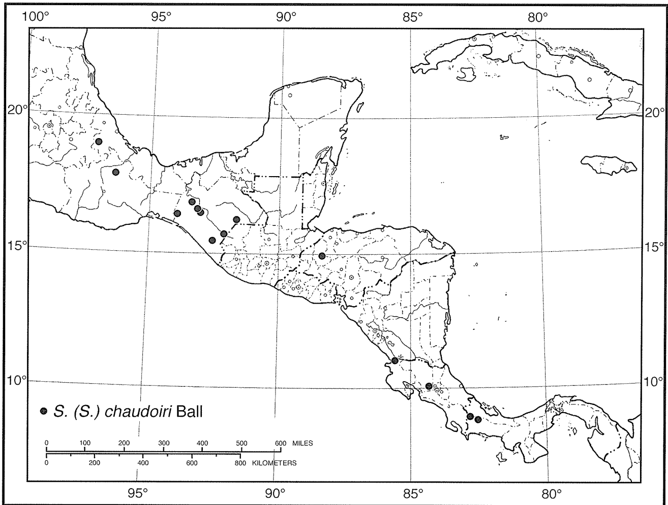
Figure 26. Map of Middle America showing positions of known localities for Stenognathus (s. str.) chaudiroides Ball.
